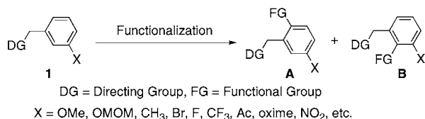
Scheme 1. Possible Products from C–H Activation/Functionalization of meta -Substituted Arenes
