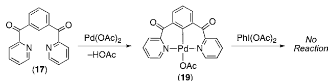
Scheme 2. Synthesis and Stoichiometric Reaction of 19 with PhI(OAc) 2
